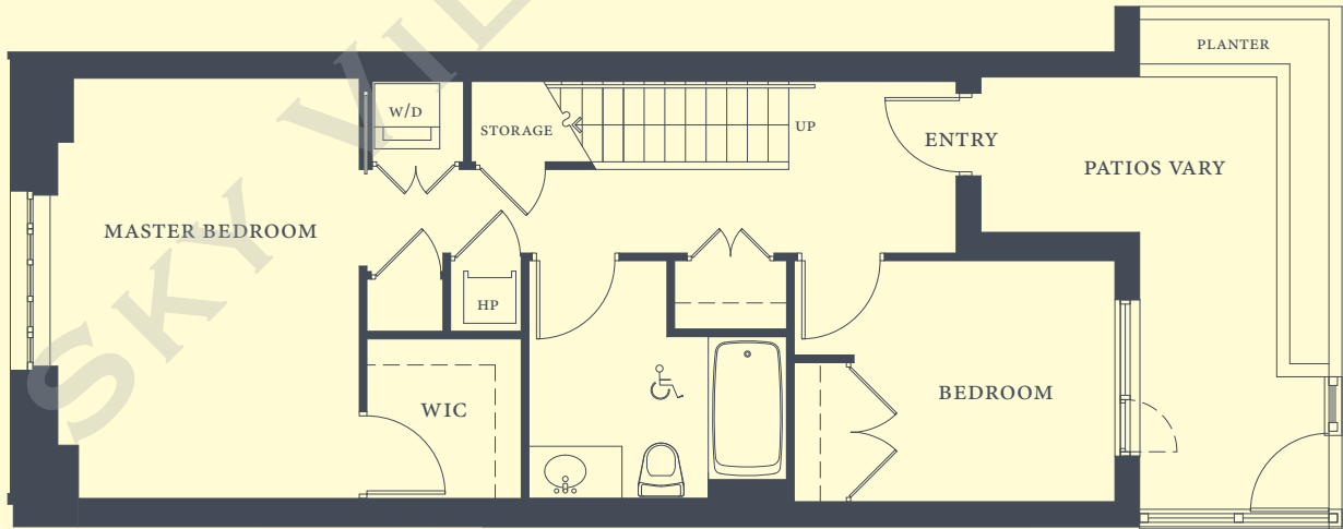
LEVEL ONE
