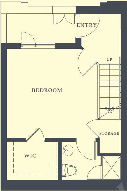
LEVEL ONE
