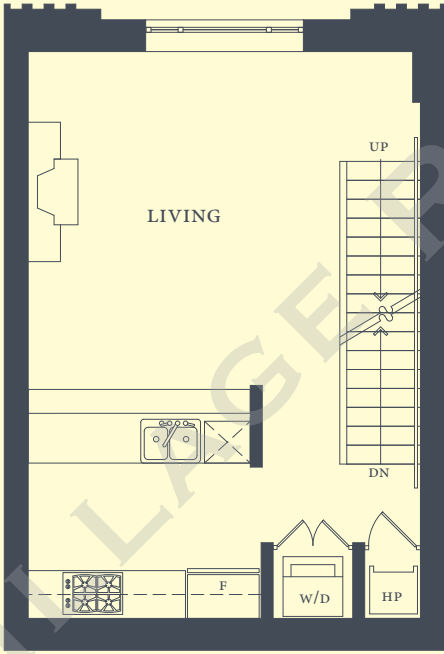
LEVEL TWO
